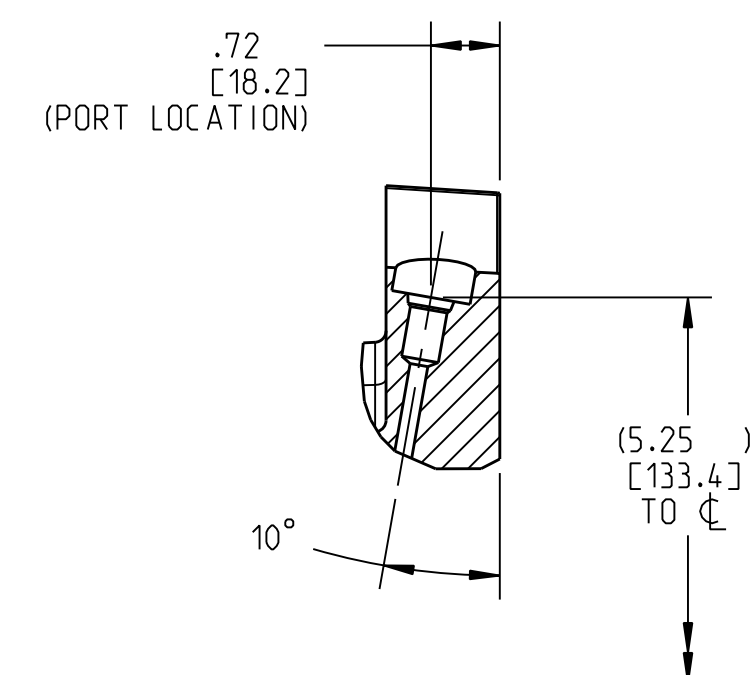
SECTION D-D 2 PLACES
