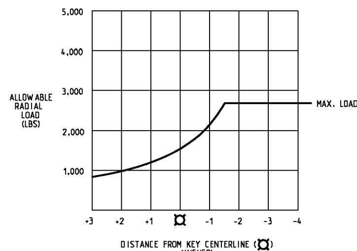
LOAD CAPACITY @ 240 RPM AND B10 = 3,000 HRS
