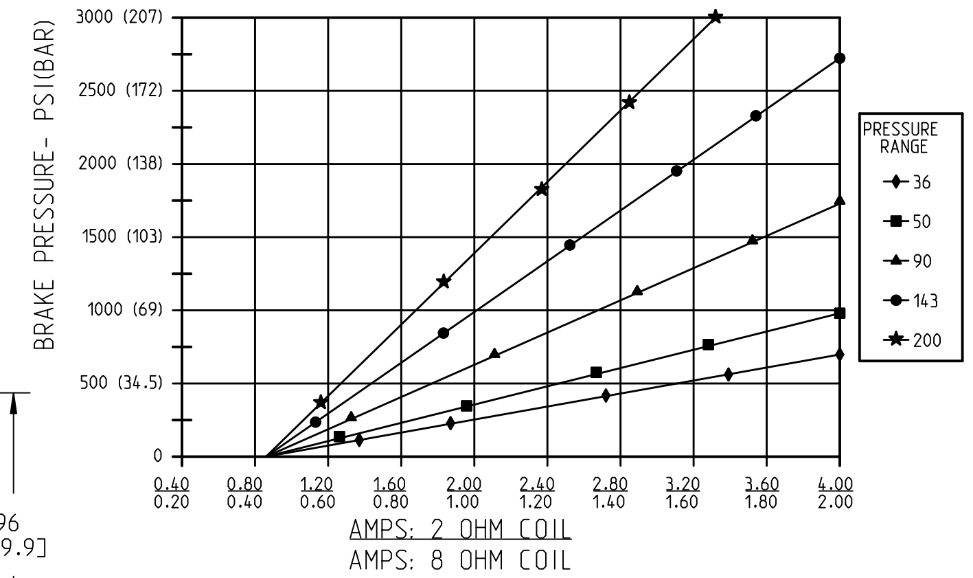
EBV-M BRAKE PRESSURE VS CURRENT
